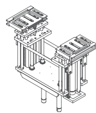
Outside ejector / 托模裝置
