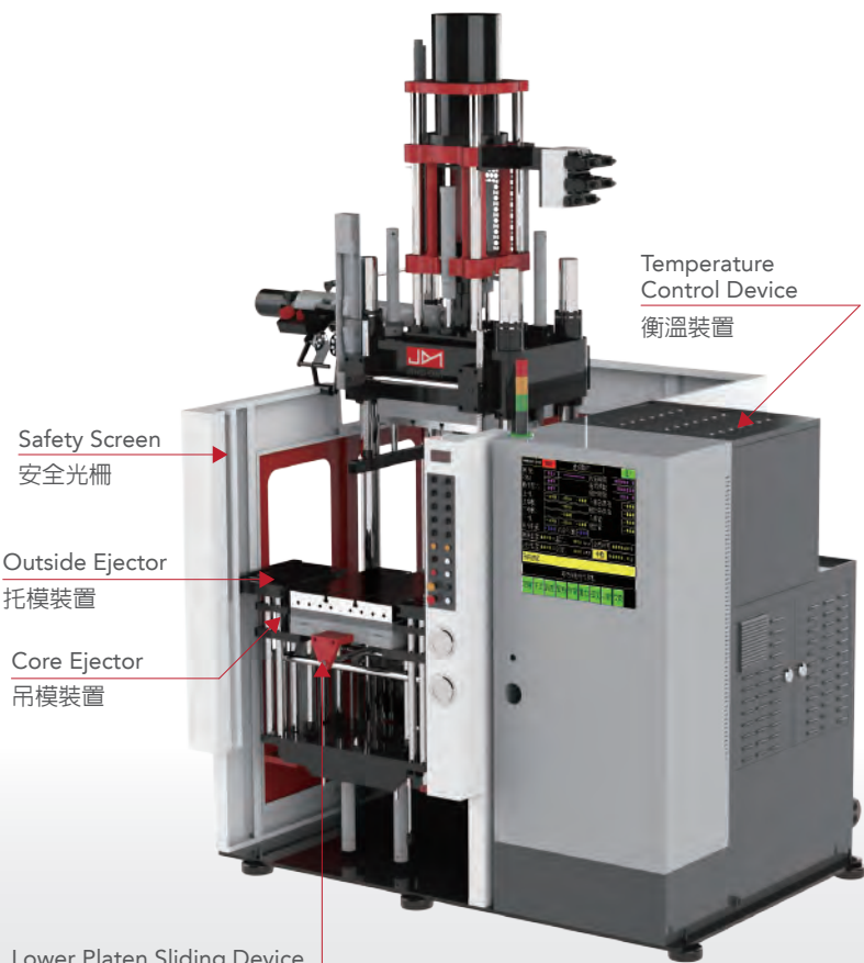
Lower Platen Sliding Device 出入模裝置
